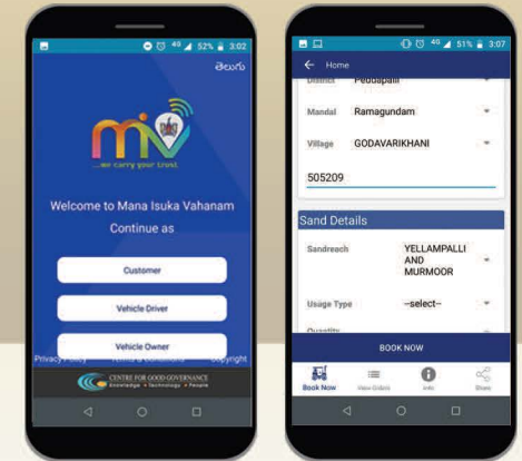
Landing Page
